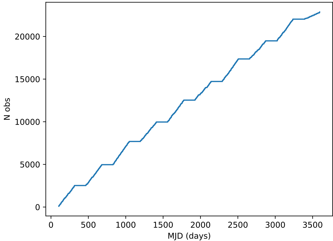
too_elab_2yr_r64_d2_ugrizy_v3.4_10yrs all bands: DD:EDFS Cumulative NVisits
