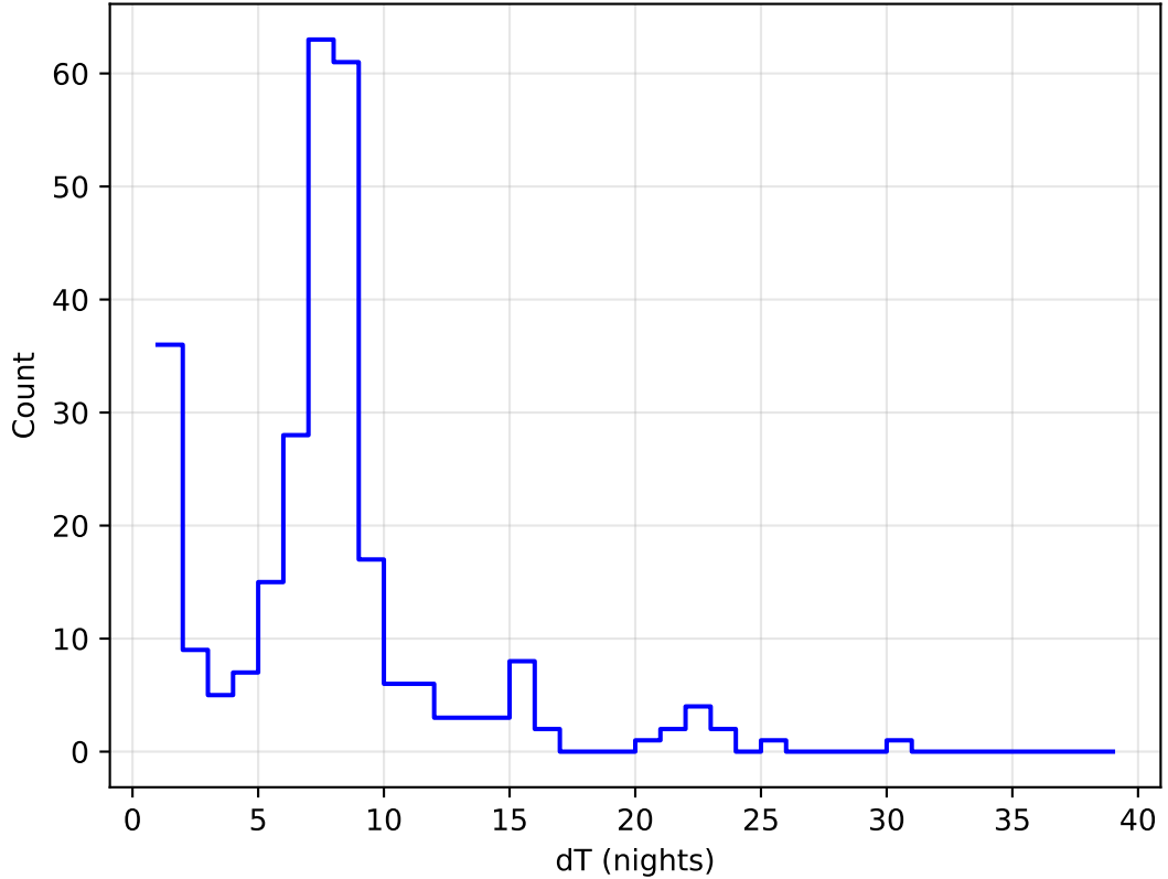
too_elab_2yr_r64_d2_ugrizy_v3.4_10yrs all bands: DD:ECDFS Delta Nights Histogram
