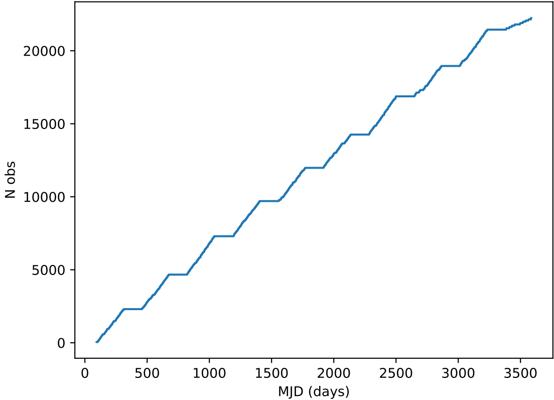
too_elab_2yr_r64_d2_ugrizy_v3.4_10yrs all bands: DD:ECDFS Cumulative NVisits
