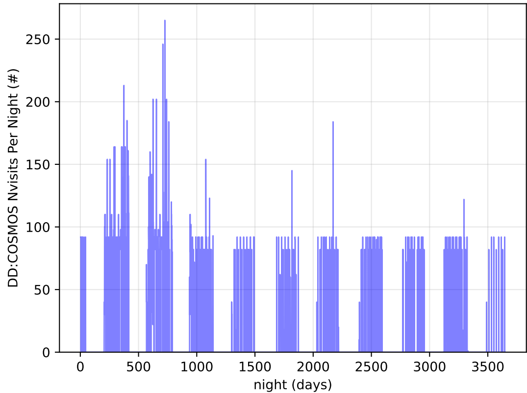
too_elab_2yr_r64_d2_ugrizy_v3.4_10yrs all bands: DD: COSMOS Nvisits Per Night
