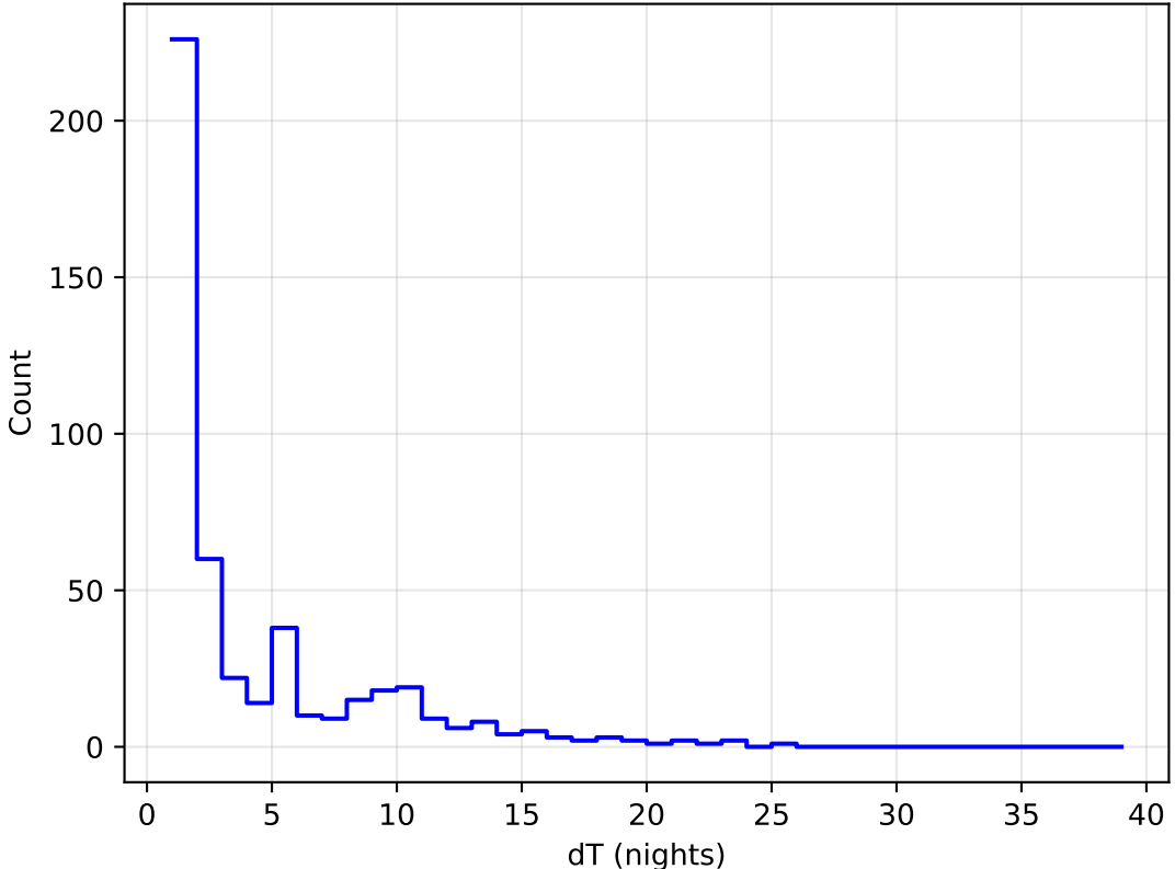
too_elab_2yr_r64_d2_ugrizy_v3.4_10yrs all bands: DD: COSMOS Delta Nights Histogram
