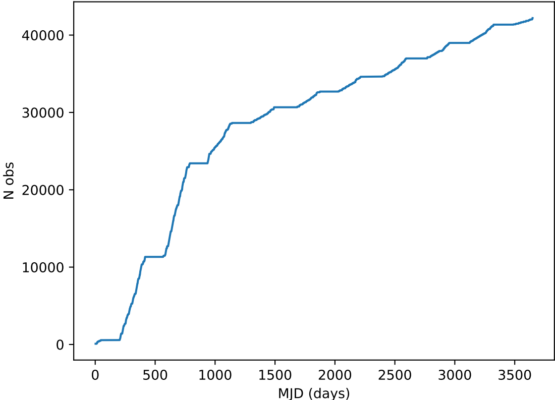
too_elab_2yr_r64_d2_ugrizy_v3.4_10yrs all bands: DD: COSMOS Cumulative NVisits
