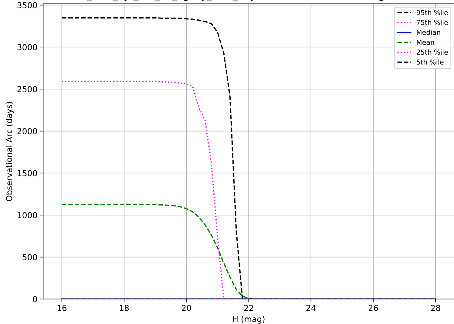
too_elab_2yr_r32_d3_ugrizy_v3.4_10yrs: Observational Arc Length Vatra
