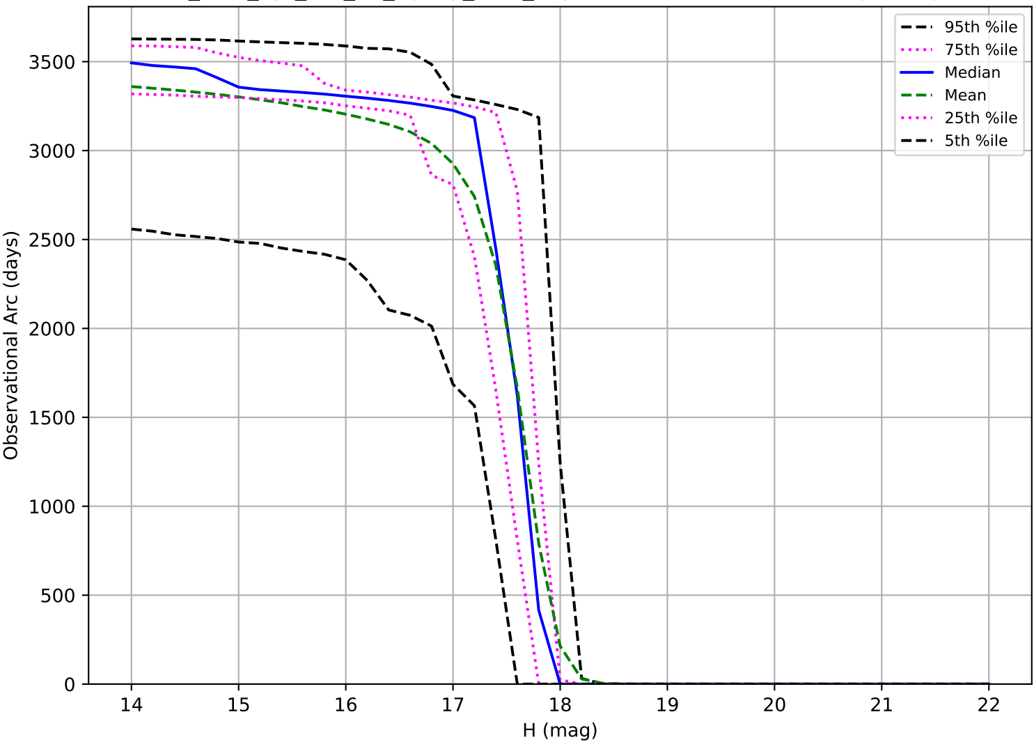
too_elab_2yr_r32_d3_ugrizy_v3.4_10yrs: Observational Arc Length Trojan
