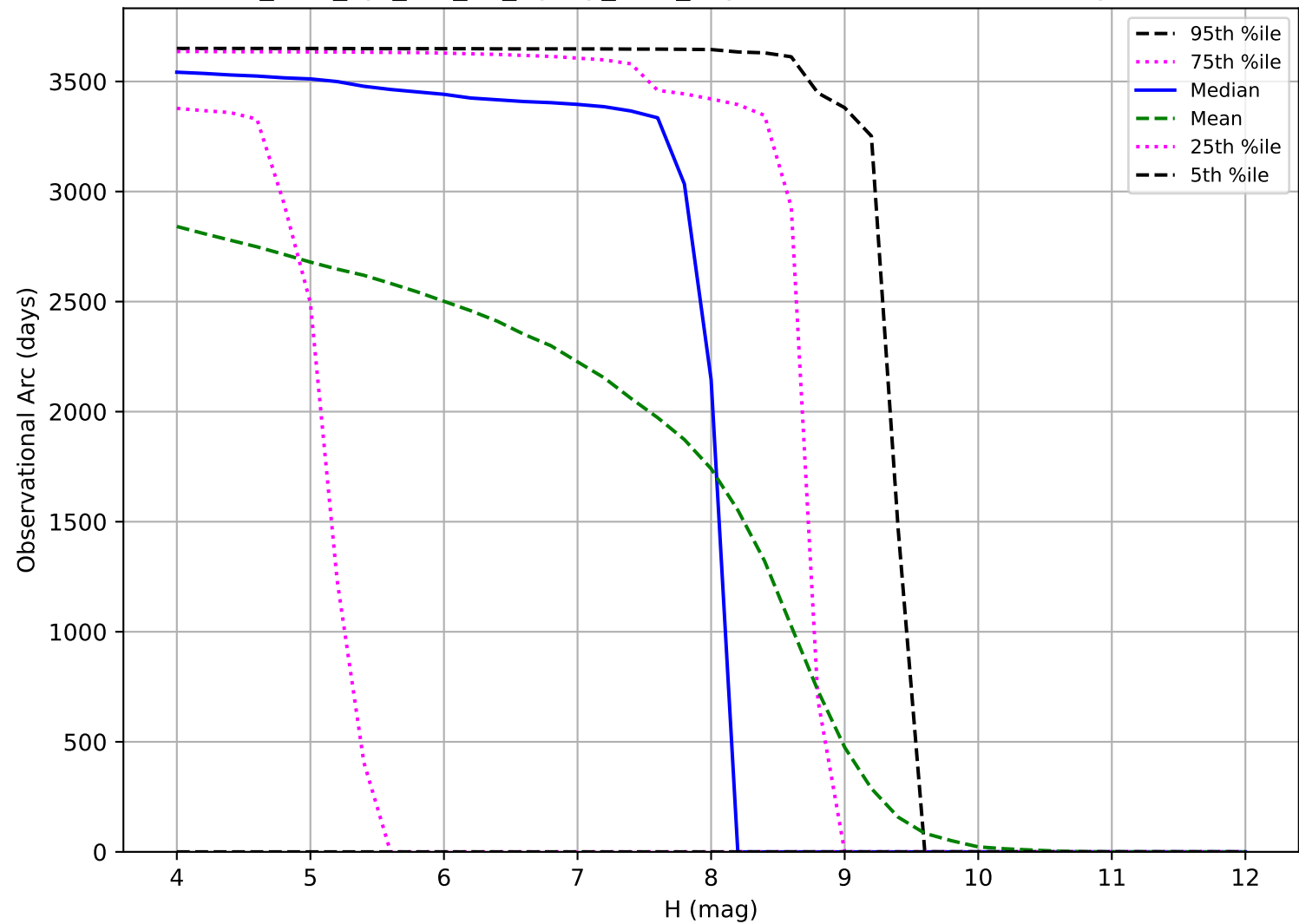
too_elab_2yr_r32_d3_ugrizy_v3.4_10yrs: Observational Arc Length TNO
