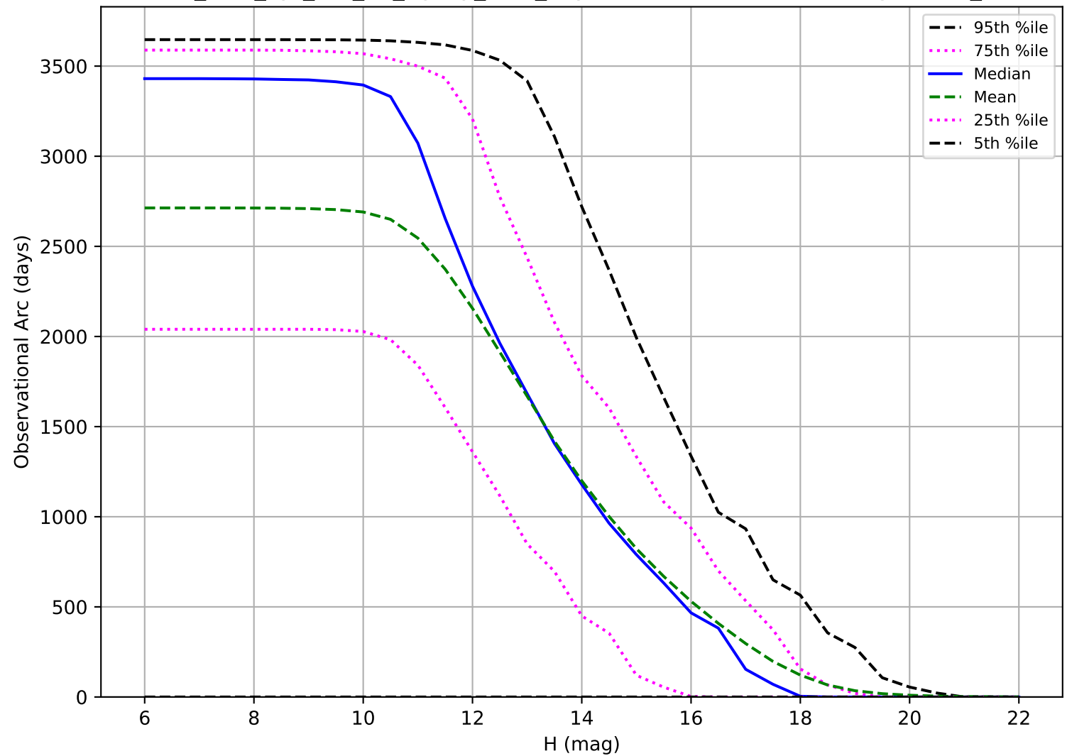
too_elab_2yr_r32_d3_ugrizy_v3.4_10yrs: Observational Arc Length OCC_r5
