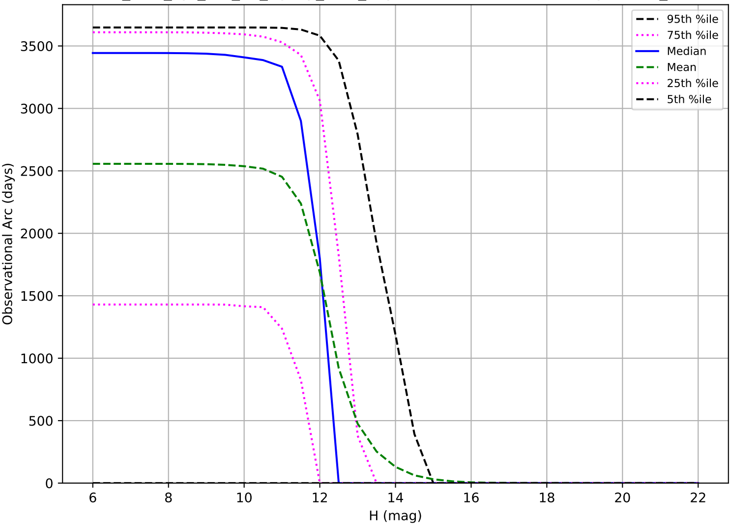
too_elab_2yr_r32_d3_ugrizy_v3.4_10yrs: Observational Arc Length OCC_r20
