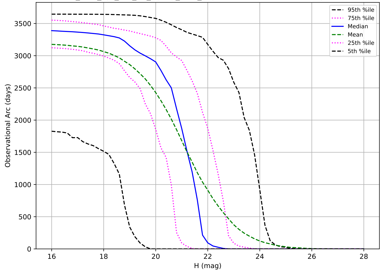
too_elab_2yr_r32_d3_ugrizy_v3.4_10yrs: Observational Arc Length NEO
