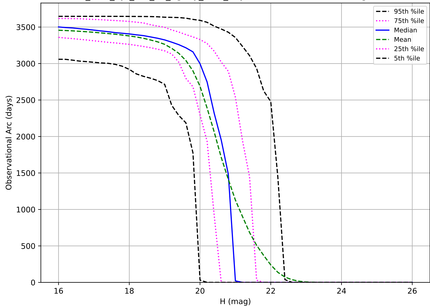
too_elab_2yr_r32_d3_ugrizy_v3.4_10yrs: Observational Arc Length MBA
