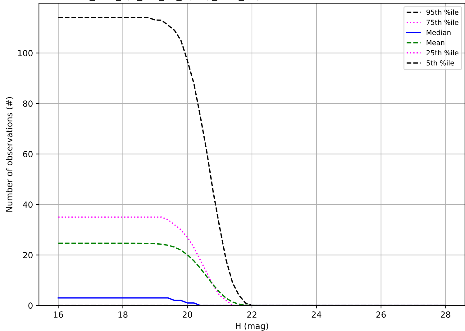
too_elab_2yr_r32_d3_ugrizy_v3.4_10yrs: Number of observations Vatira
