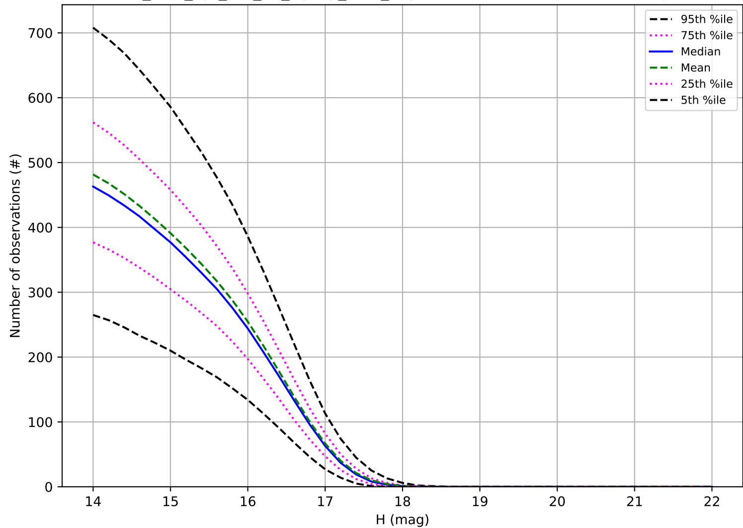
too_elab_2yr_r32_d3_ugrizy_v3.4_10yrs: Number of observations Trojan
