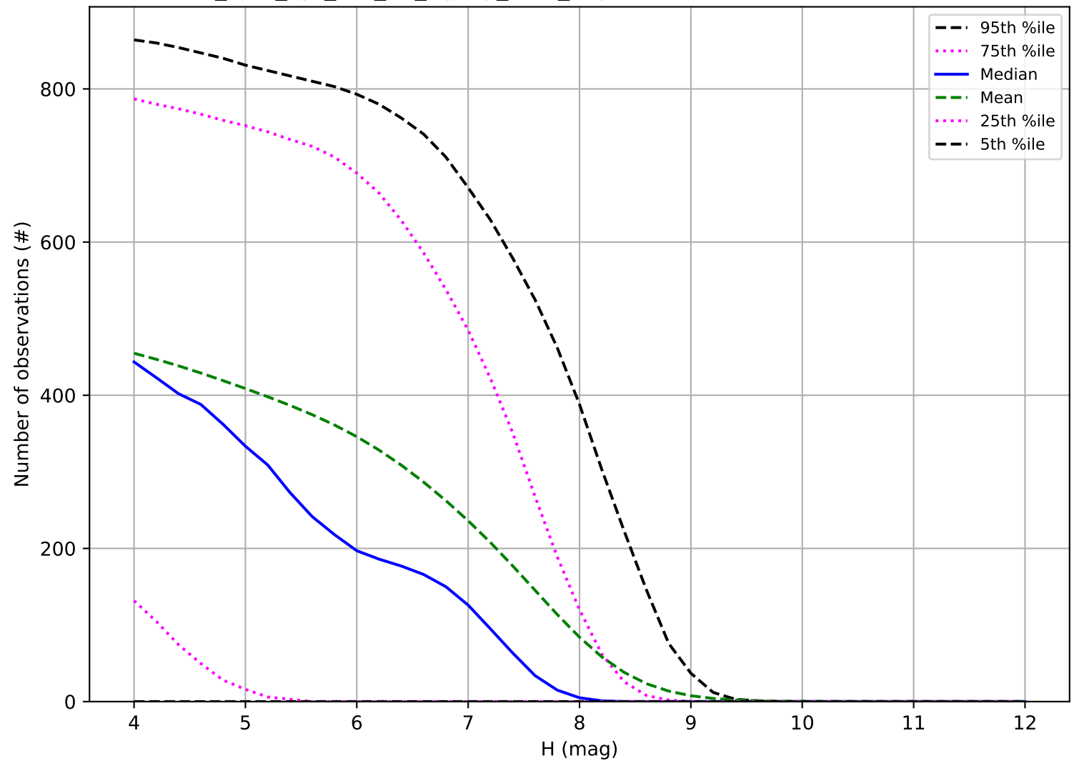
too_elab_2yr_r32_d3_ugrizy_v3.4_10yrs: Number of observations TNO
