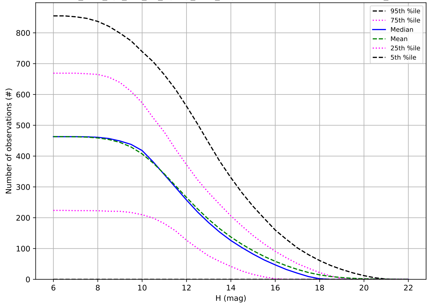
too_elab_2yr_r32_d3_ugrizy_v3.4_10yrs: Number of observations OCC_r5
