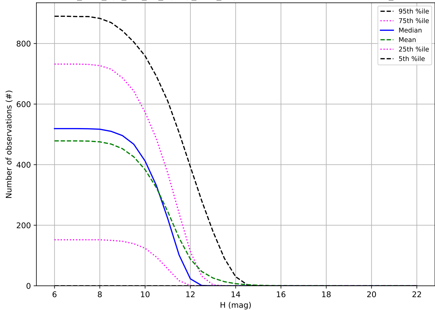
too_elab_2yr_r32_d3_ugrizy_v3.4_10yrs: Number of observations OCC_r20
