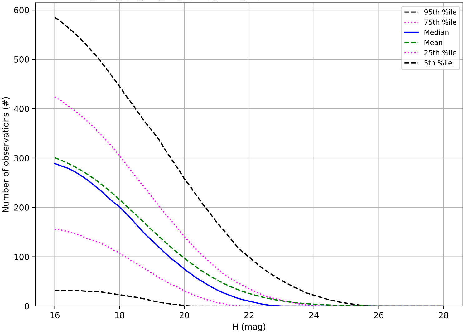
too_elab_2yr_r32_d3_ugrizy_v3.4_10yrs: Number of observations NEO
