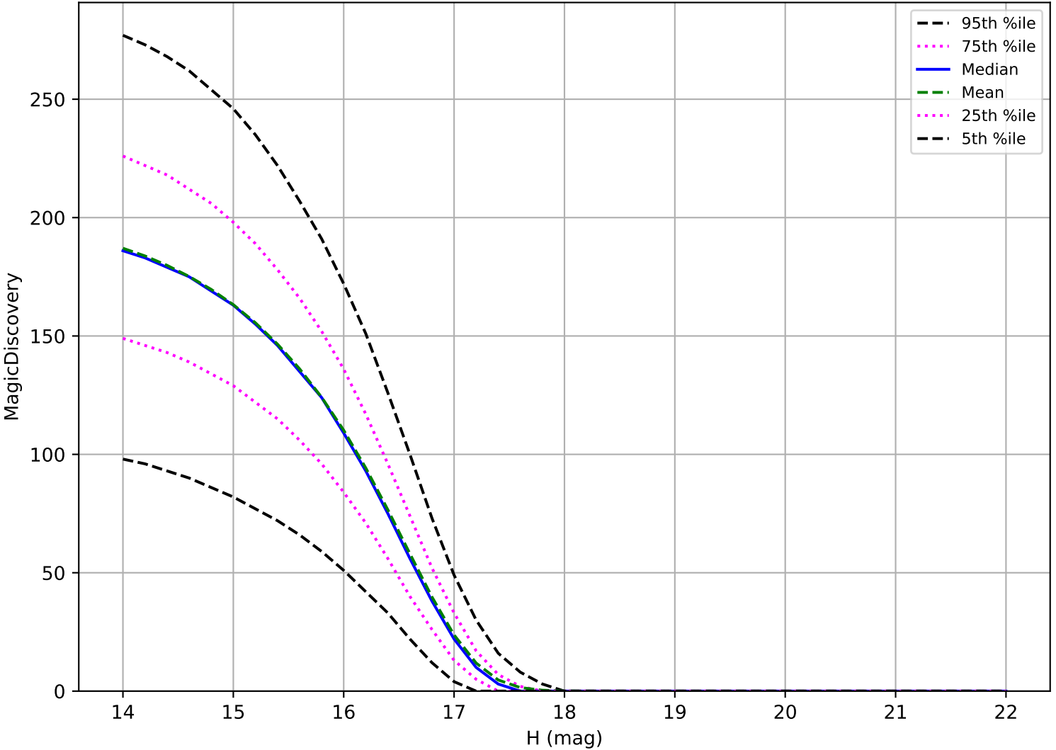
too_elab_2yr_r32_d3_ugrizy_v3.4_10yrs: Trojan 6 detections in 60 nights detection loss
