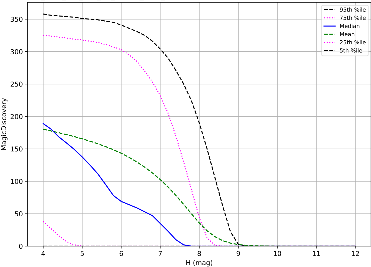
too_elab_2yr_r32_d3_ugrizy_v3.4_10yrs: TNO 6 detections in 60 nights detection loss
