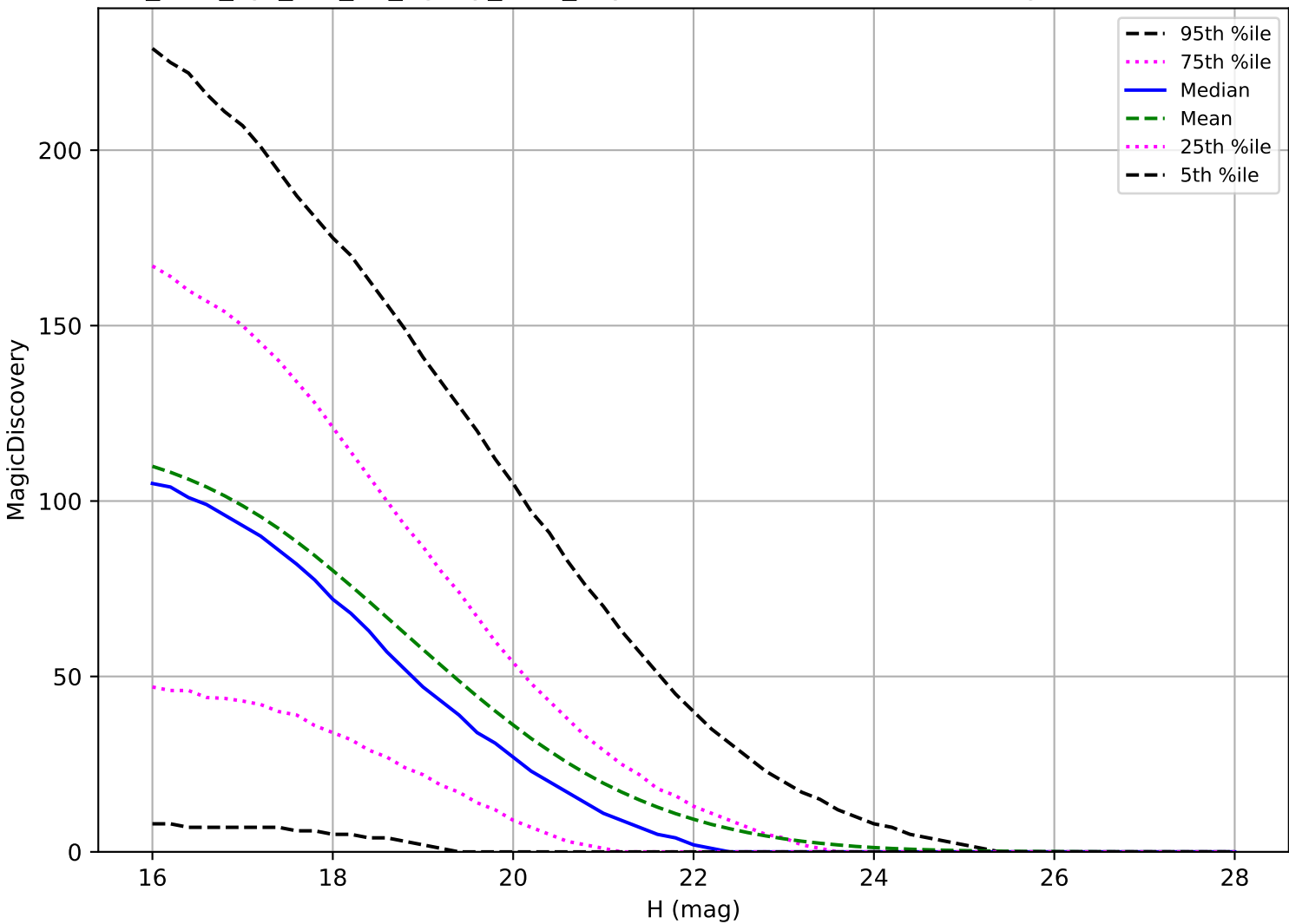
too_elab_2yr_r32_d3_ugrizy_v3.4_10yrs: PHA 6 detections in 60 nights detection loss
