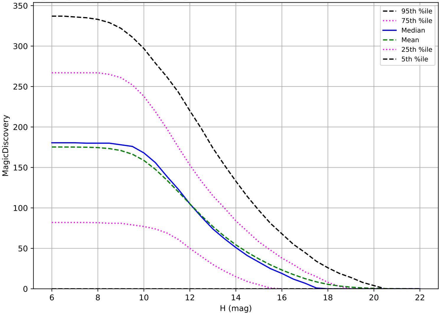
too_elab_2yr_r32_d3_ugrizy_v3.4_10yrs: OCC_r5 6 detections in 60 nights detection loss
