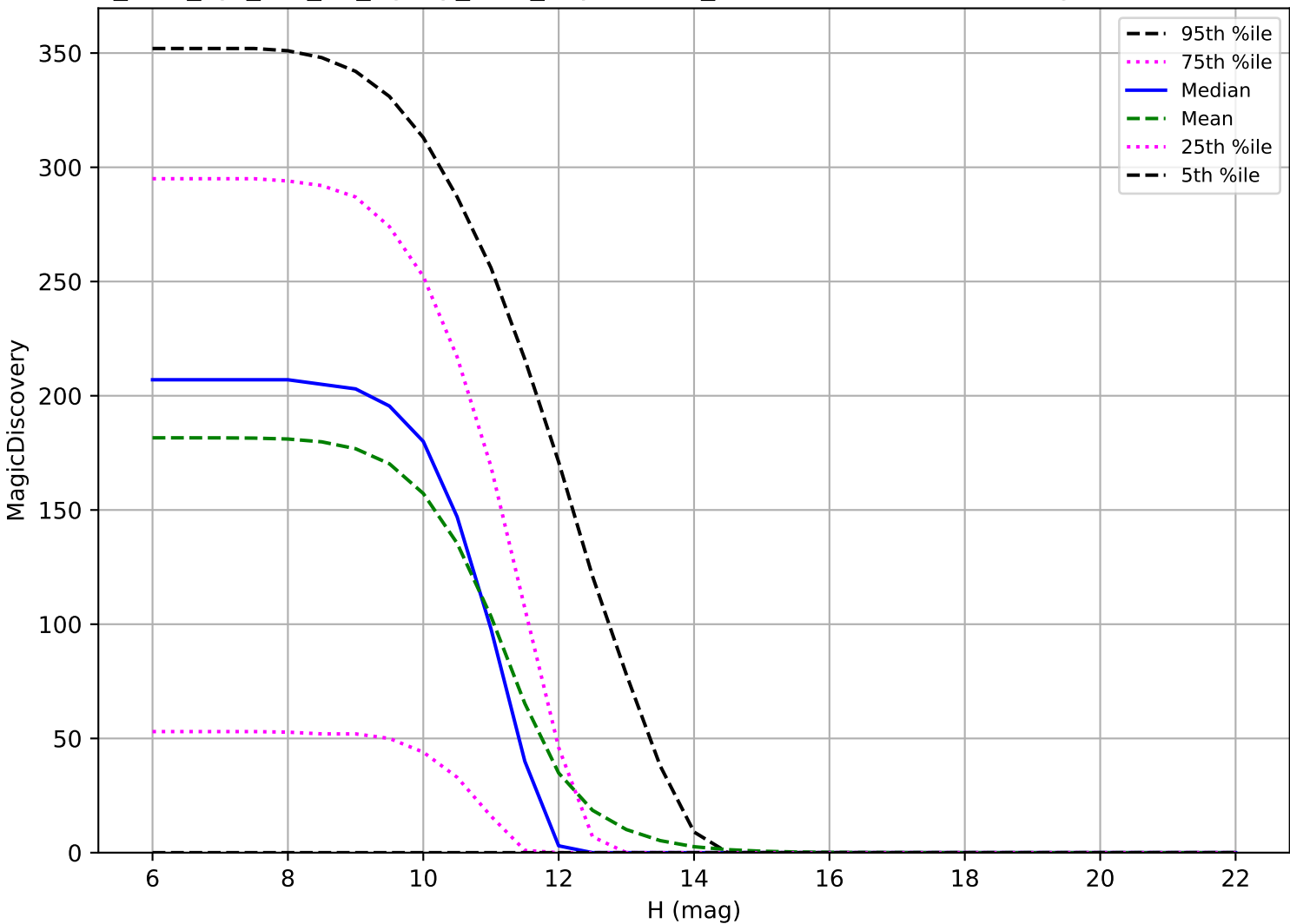
too_elab_2yr_r32_d3_ugrizy_v3.4_10yrs: OCC_r20 6 detections in 60 nights detection loss
