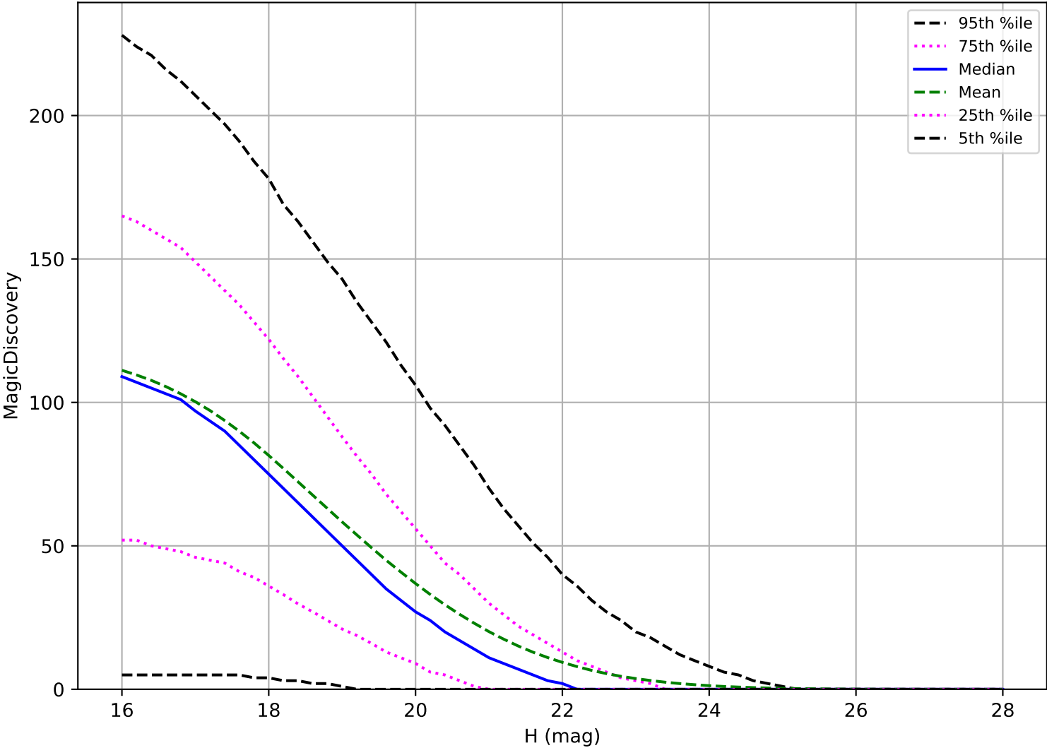
too_elab_2yr_r32_d3_ugrizy_v3.4_10yrs: NEO 6 detections in 60 nights detection loss
