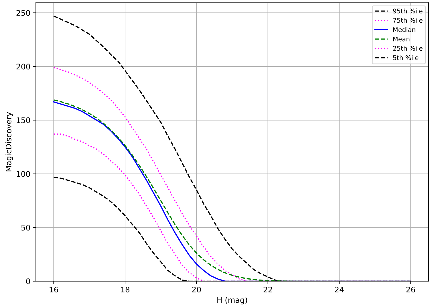
too_elab_2yr_r32_d3_ugrizy_v3.4_10yrs: MBA 6 detections in 60 nights detection loss
