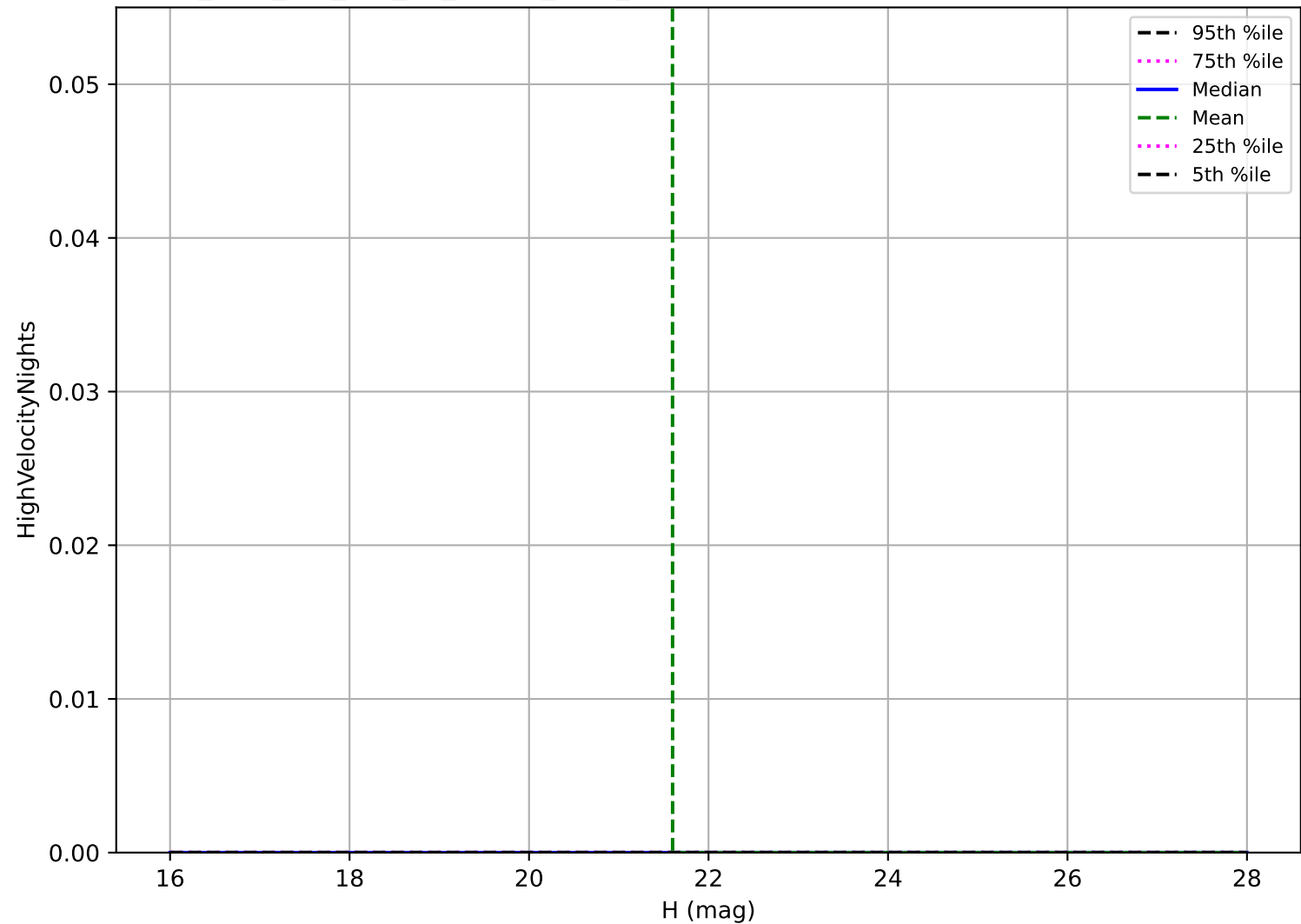
too_elab_2yr_r32_d3_ugrizy_v3.4_10yrs: Vatira High velocity pair detection loss
