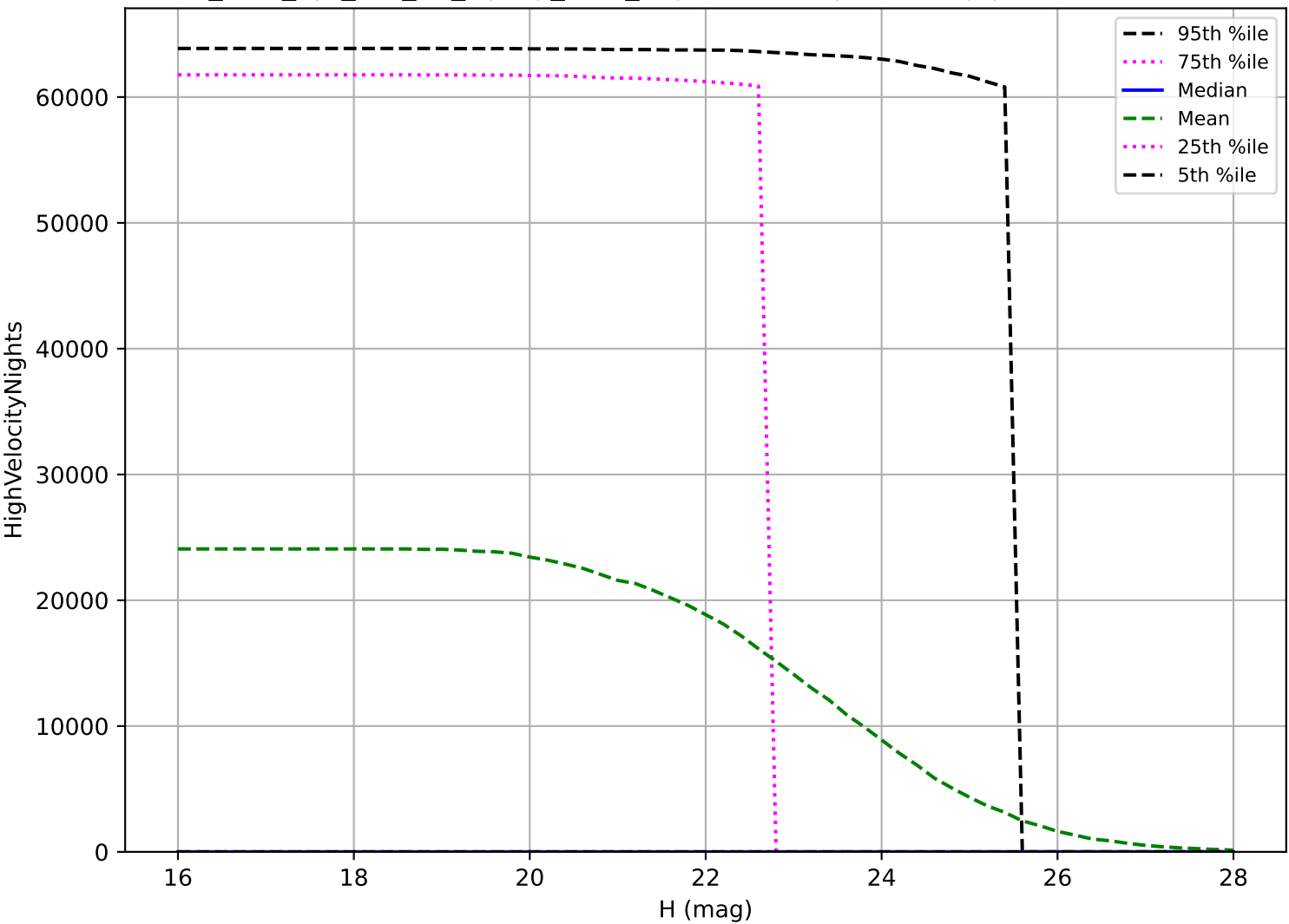
too_elab_2yr_r32_d3_ugrizy_v3.4_10yrs: PHA High velocity pair detection loss
