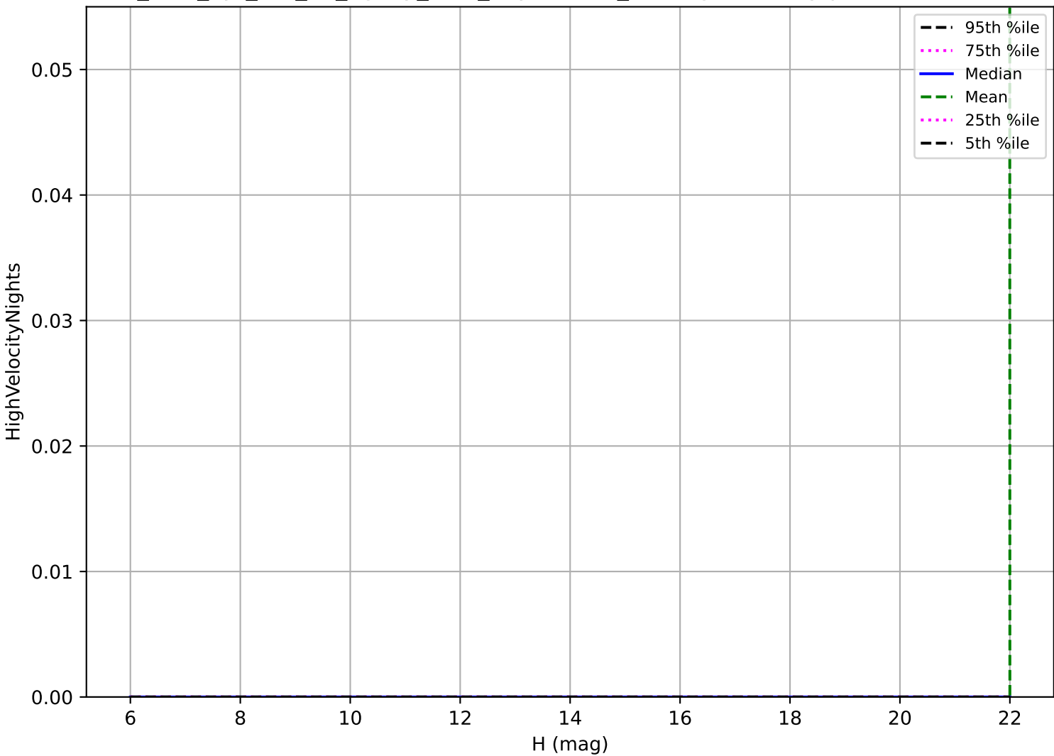
too_elab_2yr_r32_d3_ugrizy_v3.4_10yrs: OCC_r20 High velocity pair detection loss
