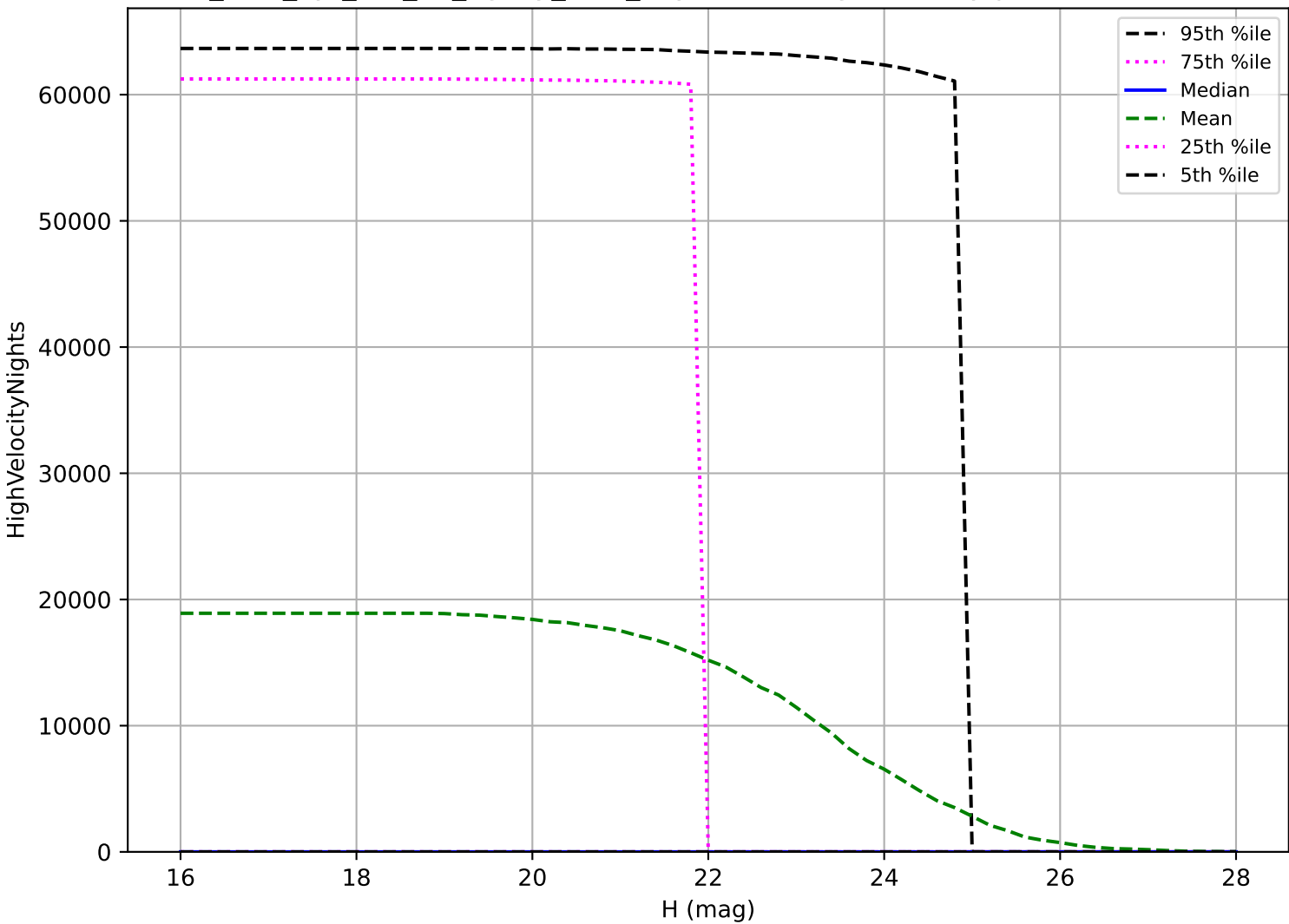
too_elab_2yr_r32_d3_ugrizy_v3.4_10yrs: NEO High velocity pair detection loss
