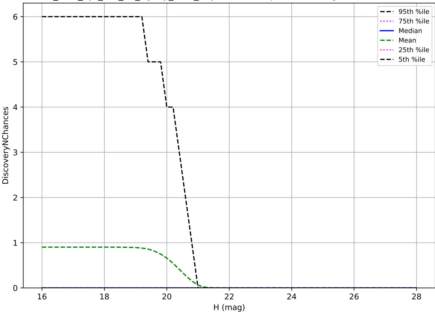
too_elab_2yr_r32_d3_ugrizy_v3.4_10yrs: Vatira 3 pairs in 15 nights detection loss
