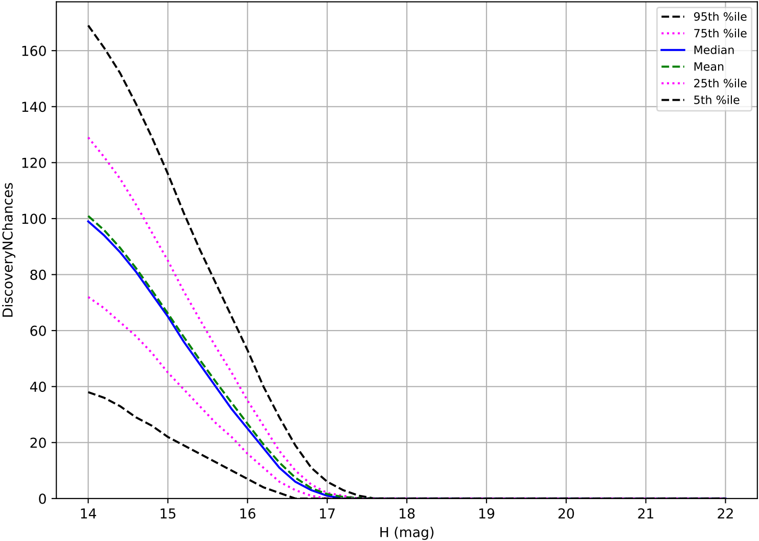
too_elab_2yr_r32_d3_ugrizy_v3.4_10yrs: Trojan 3 pairs in 15 nights detection loss
