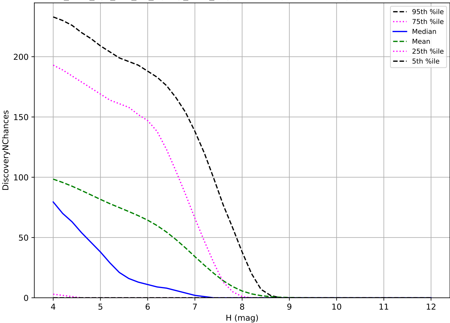
too_elab_2yr_r32_d3_ugrizy_v3.4_10yrs: TNO 3 pairs in 15 nights detection loss
