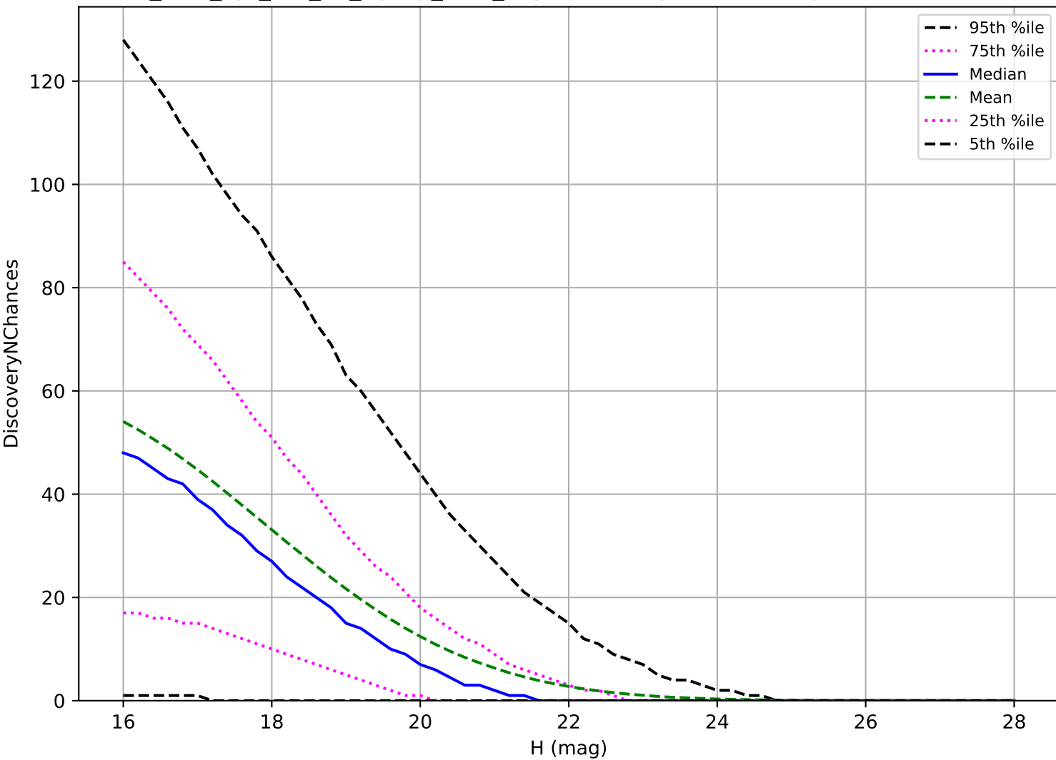
too_elab_2yr_r32_d3_ugrizy_v3.4_10yrs: PHA 3 pairs in 15 nights detection loss
