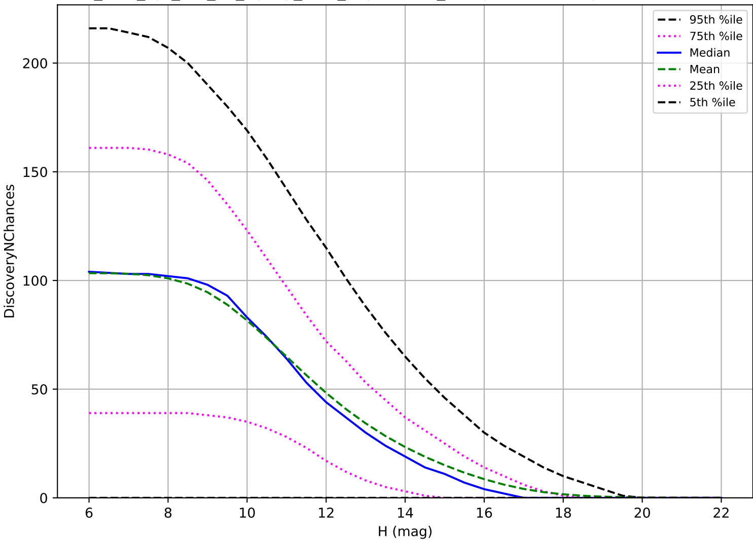
too_elab_2yr_r32_d3_ugrizy_v3.4_10yrs: OCC_r5 3 pairs in 15 nights detection loss
