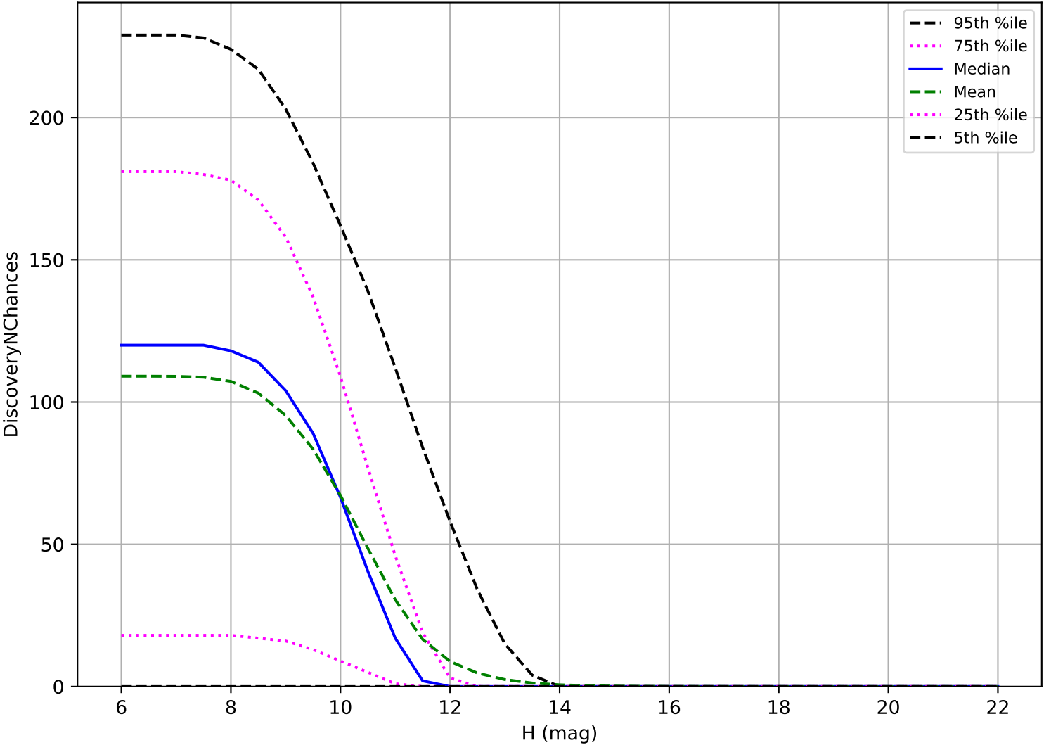
too_elab_2yr_r32_d3_ugrizy_v3.4_10yrs: OCC_r20 3 pairs in 15 nights detection loss
