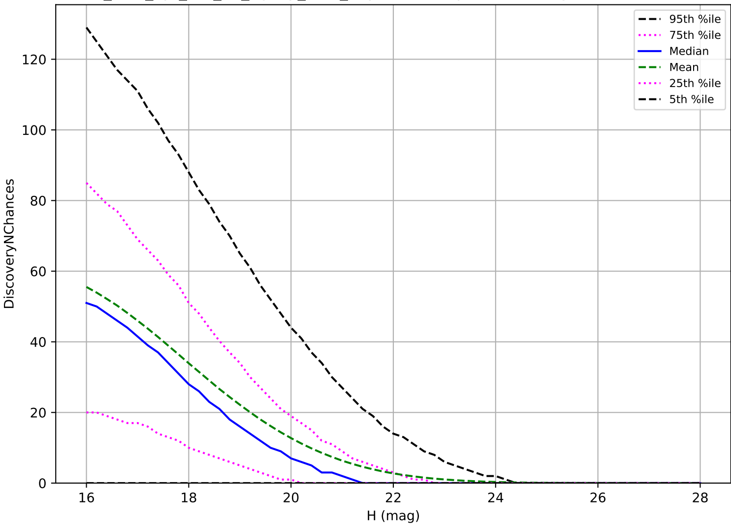
too_elab_2yr_r32_d3_ugrizy_v3.4_10yrs: NEO 3 pairs in 15 nights detection loss
