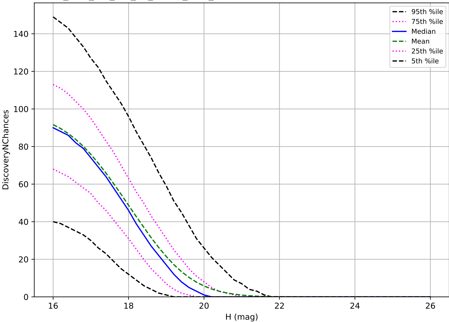
too_elab_2yr_r32_d3_ugrizy_v3.4_10yrs: MBA 3 pairs in 15 nights detection loss
