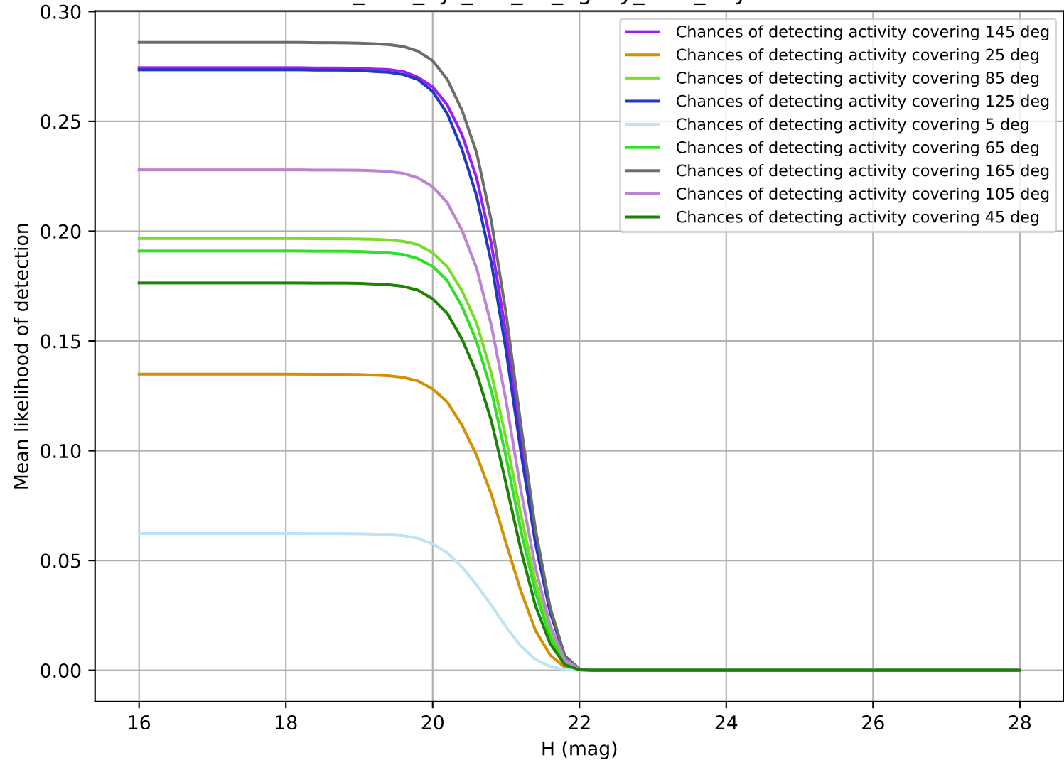
too_elab_2yr_r32_d3_ugrizy_v3.4_10yrs Vatira
