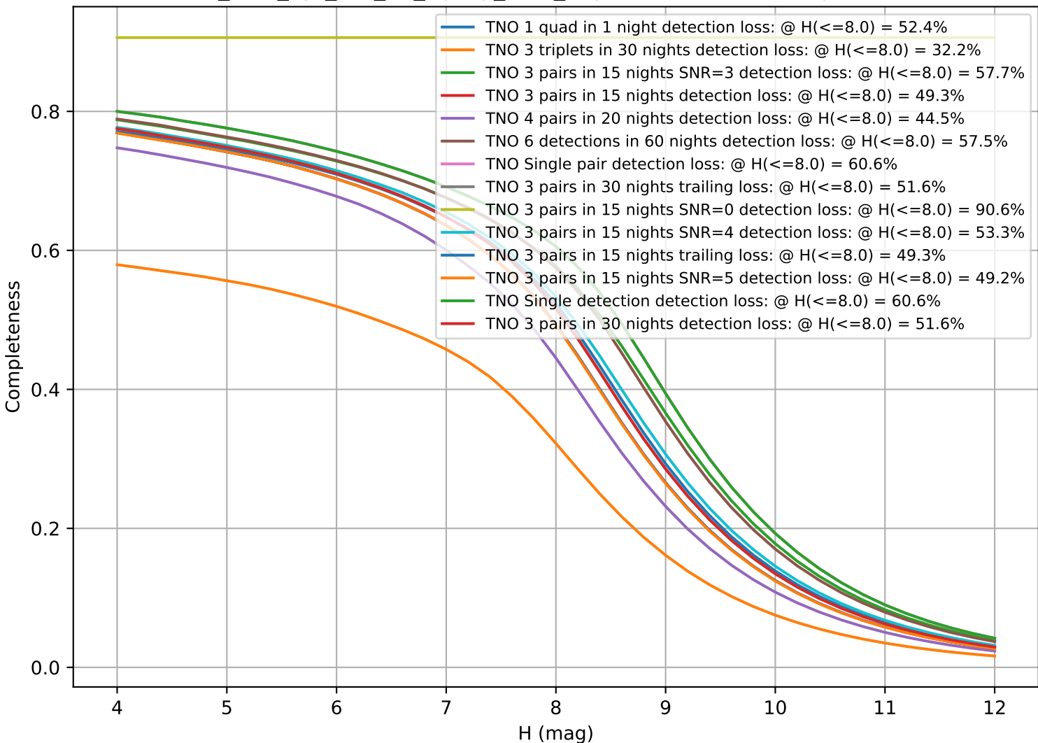
too_elab_2yr_r32_d3_ugrizy_v3.4_10yrs: CumulativeCompleteness
