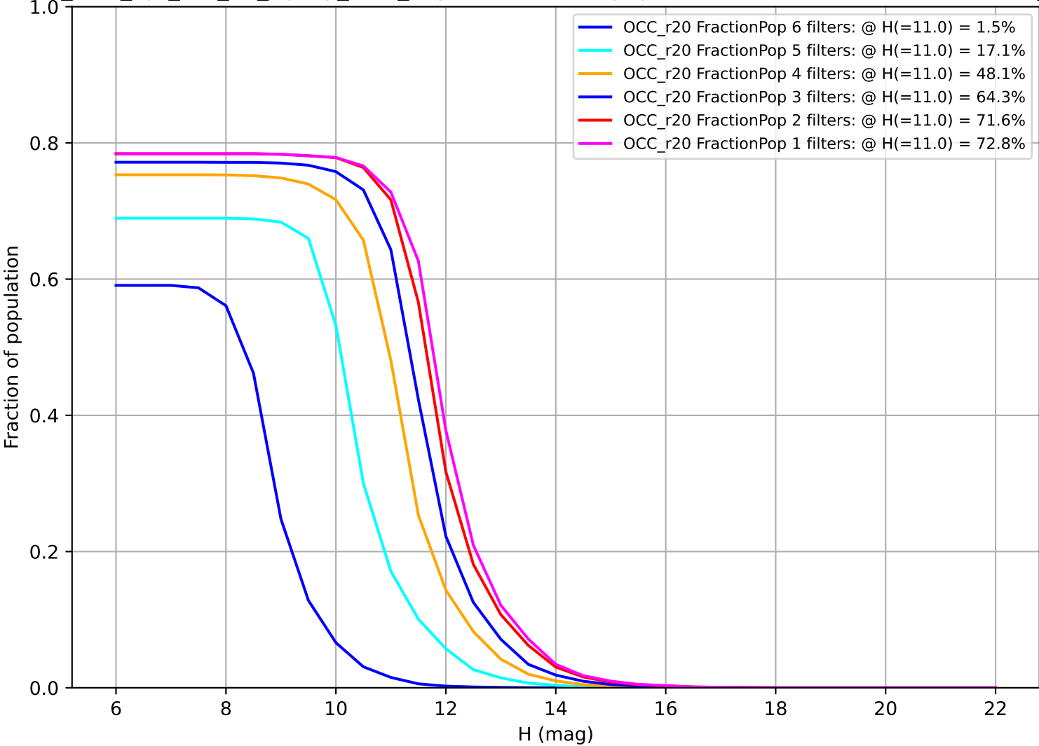
too_elab_2yr_r32_d3_ugrizy_v3.4_10yrs: Fraction of population with colors in X filters OCC_r20
