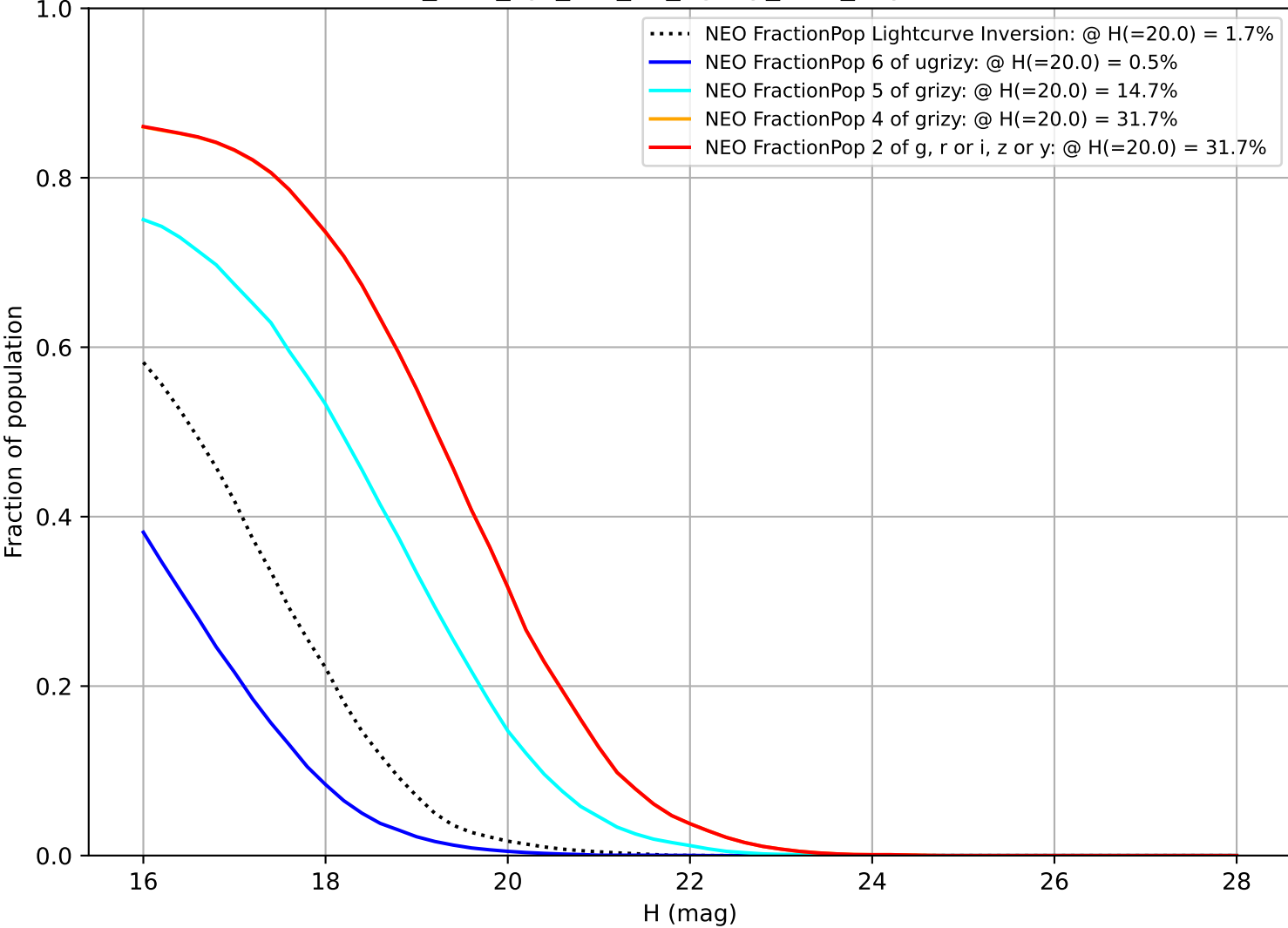
too_elab_2yr_r32_d3_ugrizy_v3.4_10yrs NEO
