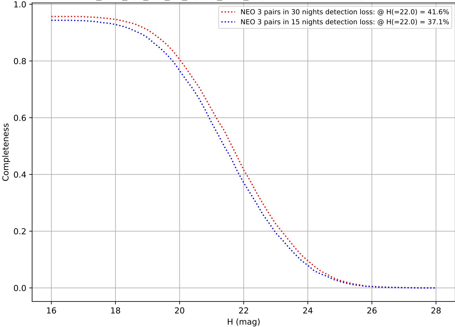
too_elab_2yr_r32_d3_ugrizy_v3.4_10yrs: DifferentialCompleteness
