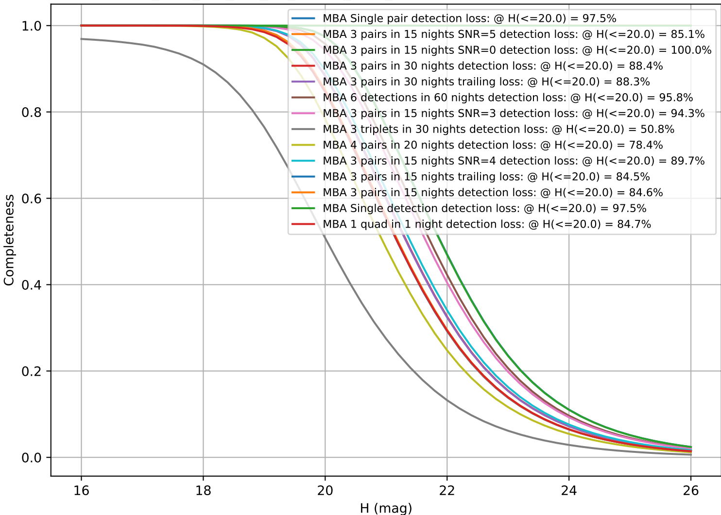
too_elab_2yr_r32_d3_ugrizy_v3.4_10yrs: CumulativeCompleteness
