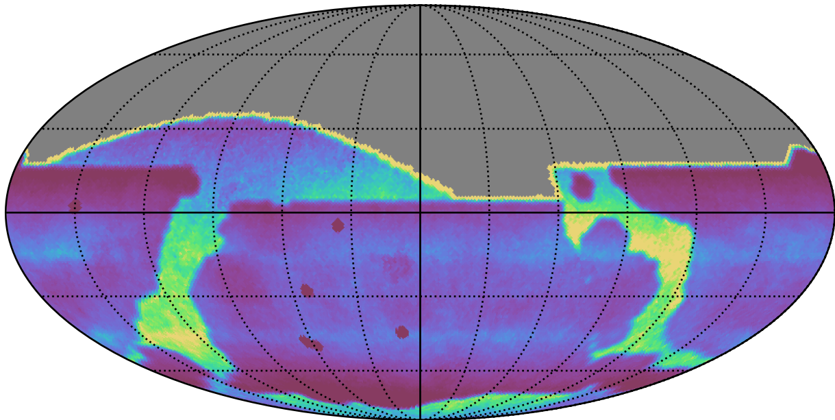
too_elab_2yr_r32_d3_ugrizy_v3.4_10yrs : DCRprecision
