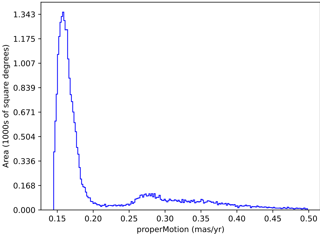
too_elab_2yr_r32_d3_ugrizy_v3.4_10yrs : properMotion
