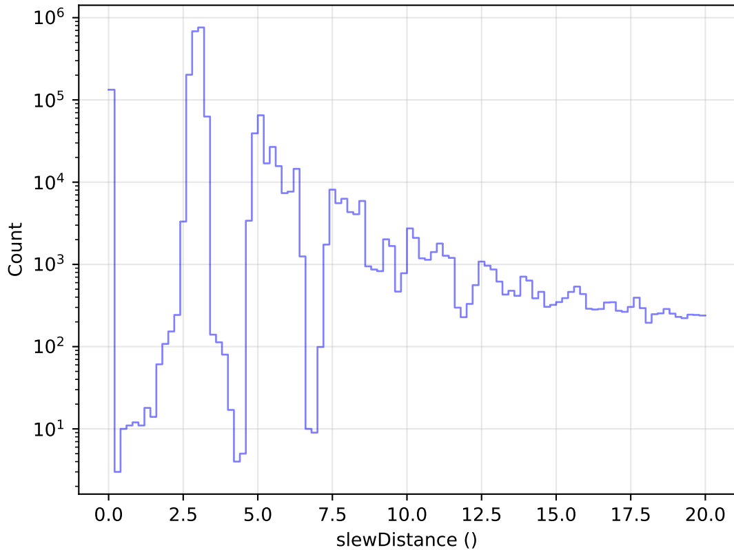
too_elab_2yr_r32_d3_ugrizy_v3.4_10yrs All visits: Zoom Slew Distance Histogram
