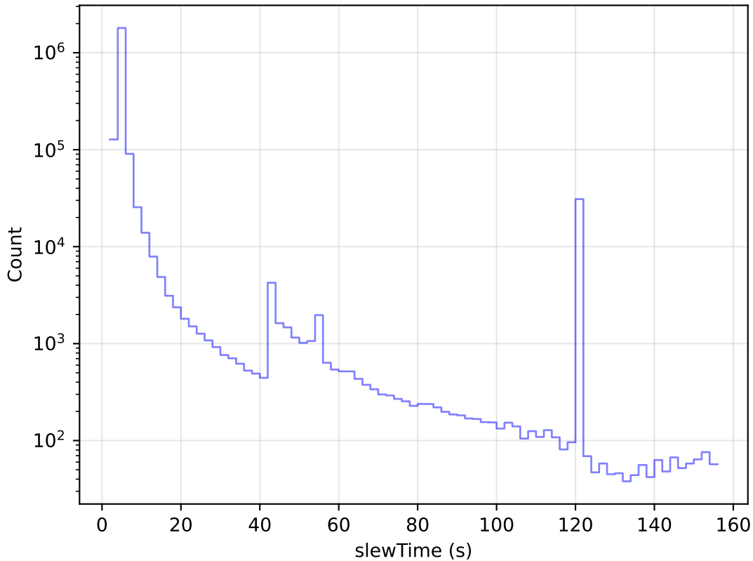
too_elab_2yr_r32_d3_ugrizy_v3.4_10yrs All visits: Slew Time Histogram
