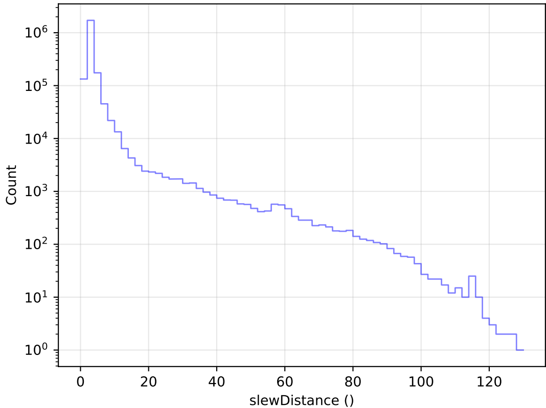
too_elab_2yr_r32_d3_ugrizy_v3.4_10yrs All visits: Slew Distance Histogram
