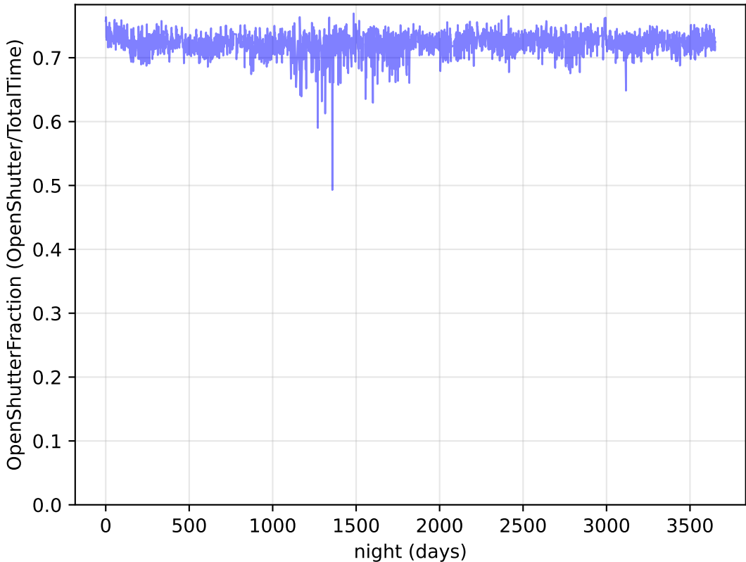
too_elab_2yr_r32_d3_ugrizy_v3.4_10yrs : OpenShutterFraction
